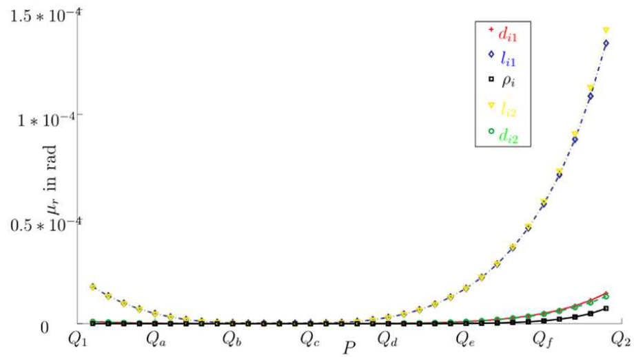
Figure 22: Sensitivity of the orientation of the end-effector to variations in geometric parameters along segment Q_1Q_2 .
