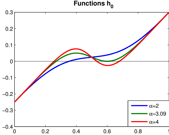
Figure 3.2: Examples of function h_0 : p_1 = 0.7 and p_2 = 0.75 and f(u) = u^\alpha . One zero for \alpha = 2 , two zeros for \alpha \approx 3.09 , three zeros for \alpha = 4 .
