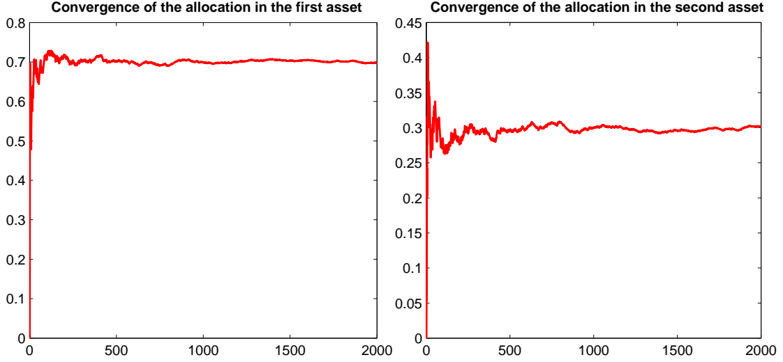
Figure 6: Convergence of \tilde{Y}_n toward y^* for f(y) = y^4 with p_1 = 0.7 and p_2 = 0.75 .
