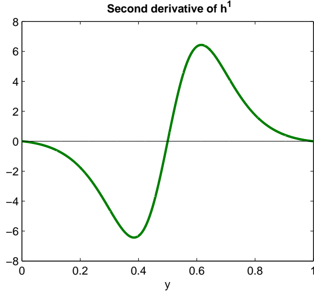
Figure 3: Second derivative of h^1 for f(y) = y^{3.09} with p_1 = 0.7 and p_2 = 0.75 .
