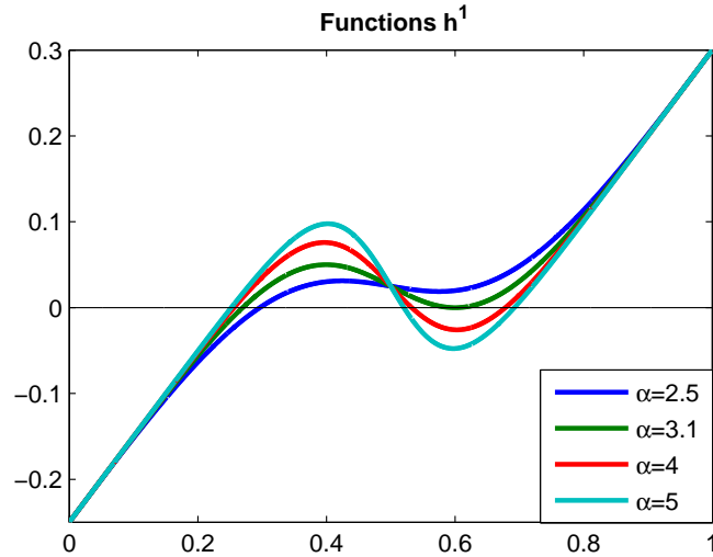
Figure 2: Functions h^1 for f(y) = y^\alpha with p_1 = 0.7 and p_2 = 0.75 .
