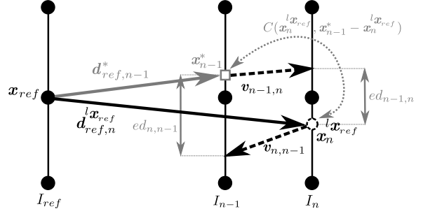
Figure 3: Matching cost and Euclidean distances ed_{n,m} and ed_{m,n} defined with respect to each temporal neighboring candidate \mathbf{x}_m^* and involved in the proposed energy. These three terms act as strong temporal smoothness constraints.
