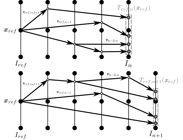
Figure 1: Multiple motion candidates are generated via a guided-random selection among all possible motion paths . This combinatorial integration (Conze et al., 2013) is done independently for each pair \{I_{ref}, I_n\} which limits the correlation between candidates selected for neighbouring frames.
