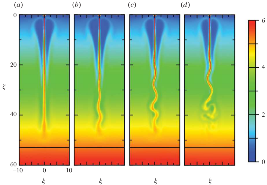
FIGURE 8. Development of the sinuous instability. Results for Re_{in}=0.05 , Sc=667 and Gr=49.05 for (a) the base flow and \tau = (b) 133.67, (c) 200.33 and (d) 250.33. The horizontal black line marks the penetration depth for the equivalent base plume flow.
