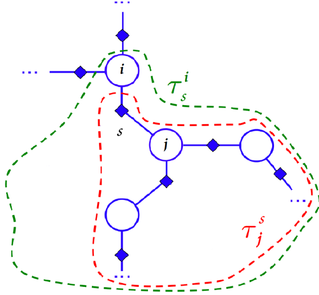
Figure 3: Examples of subtrees. This figure is partly drawn from [9].
