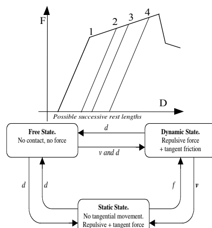
Figure 4: Up: a schematic view of the PLAST interaction. Down: finite-state automata for solid friction FROS. Transitions are made according to the variables: d: inter-mass distance; v: relative tangential speed of the two masses; f: tangent force applied
