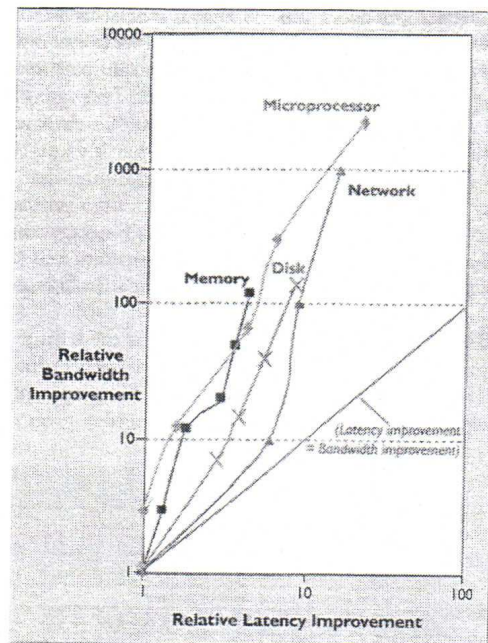
Figure 3b. Latency lags Bandwidth (from Paterson [39])
