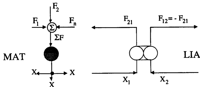
MAT and LIA : the two basic atoms of the Cordis-Anima modeller-simulator
