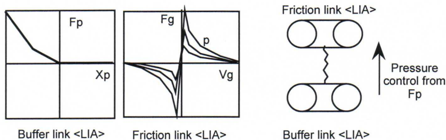
Figure 4. The friction physical module is a double non linear <LIA> : NL friction & buffer.
