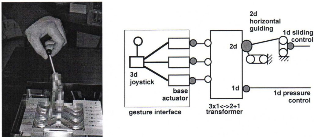
Figure 2. The 3d bowing force feedback joystick and its coupling to the bow simulation.
