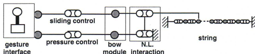
Figure 1. The bowed string model.
