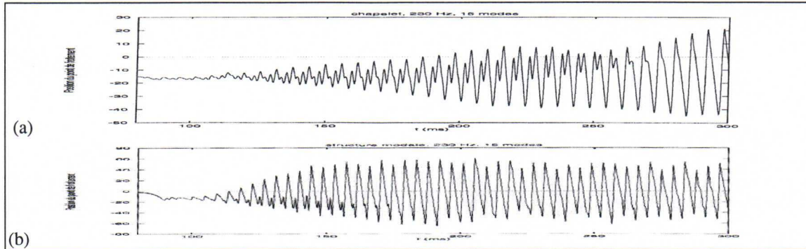
Figure 3. An attack transition of a homogeneous non-harmonic chaplet (a) and of a harmonic (b) one.
