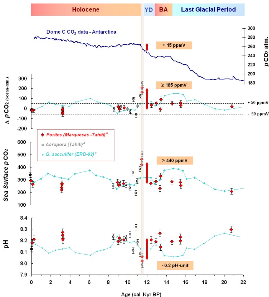
Fig. 7. Comparison of the sub-Equatorial Pacific \delta^{11}\text{B} -pH of marine biogenic carbonates over the last 21 000 cal yr. Sources are (a) this study; (b) Gaillardet and Allègre, 1995; and (c) Palmer and Pearson, 2003. Filled black diamond: modern Moorea-Tahiti Porites value published by Gaillardet and Allègre (1995). The calculation parameters for the pH are \alpha=0.981 ; \delta^{11}\text{B}_{\text{SW}}=39.9\% ; S=35\% ; and T=27^\circ\text{C} for Tahiti (Moorea) and T=28^\circ\text{C} for the Marquesas Islands and for ERDC-92. Deduced \Delta p\text{CO}_2 values (Table 1, see text) and atmospheric p\text{CO}_2 data (Monnin et al., 2001, 2004) are also plotted to illustrate the synchronization between the abrupt changes to the sea surface pH and \Delta p\text{CO}_2 in the central sub-Equatorial Pacific and the atmospheric \text{CO}_2 increase of 15–20 ppmV at the end of the YD event.
