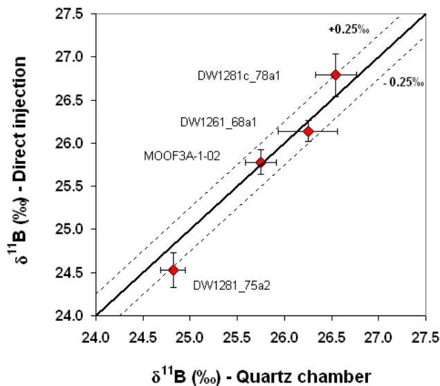
Fig. 3. Comparison of MC-ICPMS analyses using direct injection (d-DIHEN) and conventional introduction for Porites referenced DW1281c_78a1, DW1261_68a1, DW1281_75a2 and MOOF3A-1-02. \delta^{11}\text{B} results show an excellent agreement of the two introduction technique within the external reproducibility considered here of \pm 0.25\text{‰} . Error bars are the standard deviation calculated from the “n” measurements for each sample (Table 1).
