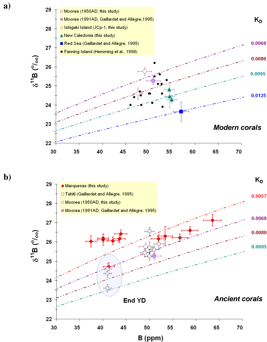
Fig. 4. The \delta^{11}\text{B} values plotted against the boron concentrations (a) for modern Porites from various geographical areas and (b) for ancient Porites and Acropora near Marquesas and the Tahiti Islands. The theoretical curves for different partition coefficient K_D values were calculated assuming T=28^\circ\text{C} ; S=35\% ; \alpha=0.981 ; and \delta^{11}\text{B}_{\text{SW}}=39.9\% . Seawater values used were [\text{B}]_{\text{seawater}}=416\ \mu\text{M} and T\text{CO}_2=2\ \text{mM} .
