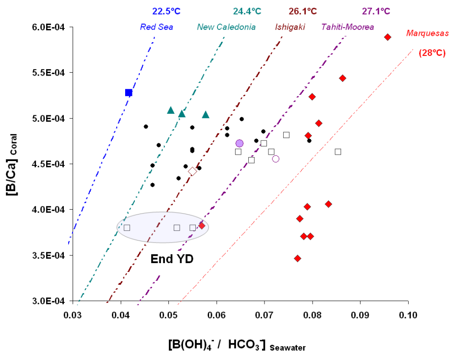
Fig. 5. B/Ca molar ratio in coral plotted against the borate/bicarbonate molar ratio in seawater. Theoretical curves for different partition coefficient K_D values were calculated assuming T=28^\circ\text{C} ; S=35\text{‰} ; \alpha=0.981 ; and \delta^{11}\text{B}_{\text{SW}}=39.9\text{‰} . Regional SSTs was used to calculate the borate/bicarbonate ratios for each of the corals. The temperature strongly influences the partition coefficient K_D . Porites near Marquesas showed a K_D of \sim 0.0057 . The seawater values used to calibrate the partition coefficient were [\text{B}]_{\text{seawater}}=416\ \mu\text{M} and T\text{CO}_2=2\ \text{mM} .
