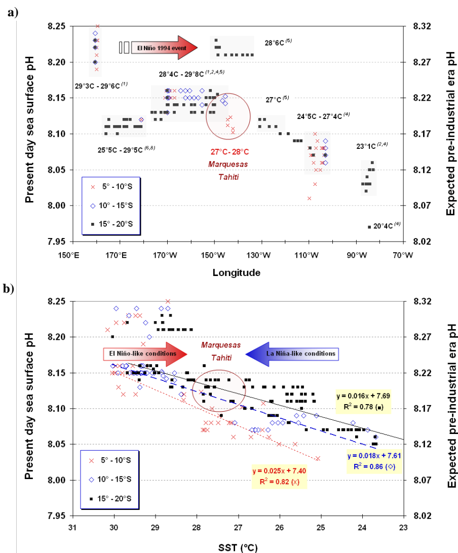
Fig. 2. (a) The present day sea surface pH in the sub-Equatorial Pacific Ocean as function of the geographical location (left axis). 0.07 pH-units are added to the present day pH on the pre-industrial era pH axis (see text). The month (values in parenthesis) of the water sampling and the averaged SSTs are also indicated. (b) Sea surface pH in the sub-Equatorial Pacific Ocean plotted against SST between 150° E and 80° W. Similar pH-SST correlations were observed for surface waters between 80° W and 170° W at three different ranges of latitude (sources from http://www.nodc.noaa.gov/OC5/SELECT/dbsearch/dbsearch.html ; measurement years: 1980–1998; depths: 0–50 m).
