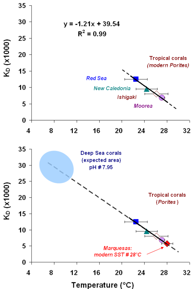
Fig. 6. Linear correlation between the mean regional SST and the partition coefficient K_D obtained from modern Porites samples collected from various SST areas. This regression shows the influence of the temperature on K_D and is valid for various aragonite species. The tropical corals are Porites , Acropora , and the cold sea coral is Lophelia pertusa . The expected area for cold sea corals (6–11 °C) was determined from pH 7.95 and from the high boron concentrations (78–100 ppm) measured in North Atlantic Lophelia pertusa samples collected between 40° N and 70° N (Douville et al., 2007).
