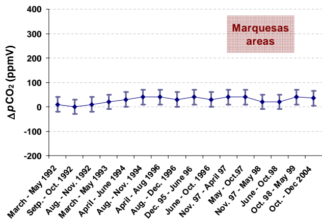
Fig. 8. The relative stability of modern \Delta p\text{CO}_2 values close to equilibrium in the Tahiti – Marquesas area between 1992 AD and 2004 AD (Dandonneau, 1995; Feely et al., 1999, 2002; Goyet et al., 2009; Goyet and Peltzer, 1997).
