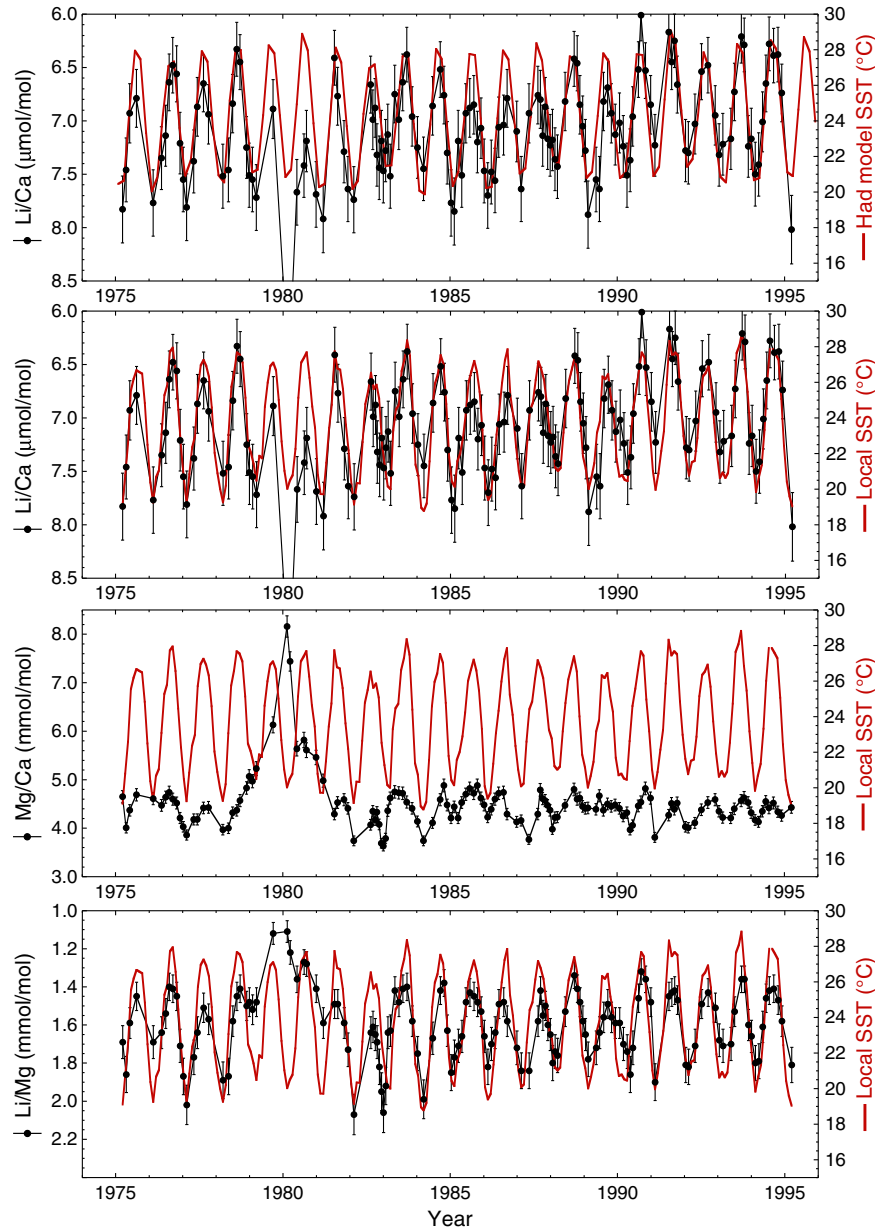
Figure 1. Li/Ca, Mg/Ca, and Li/Mg ratios for a 20 year period of a Porites coral from Ogasawara Island (OGA) compared with a gridded SST product that represents a 1^\circ \times 1^\circ area (HadISST1.1) [Rayner et al. , 2003] and locally measured SST. Error bars represent the 2\sigma external uncertainty based on repeated measurement of the JCp-1 reference material (section 2.2).
