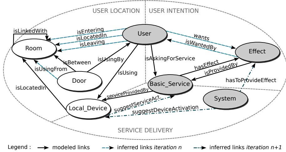
Fig. 3. Excerpt of the ontology for user location, user intention and service delivery
