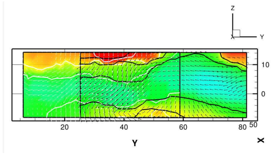
Figure 11: Comparison of the velocity fields obtained in the YZ plane with scanning (in black) and tomo-PIV (in white). The velocity fields represented are tangential and the iso-contours represents the velocity component perpendicular to the plane.
