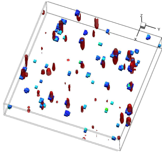
Figure 8: Comparison of the volumes (particle density corresponding to 2 grams) obtained with the scanning technique (smooth, red particles) and with Tomo-PIV (blue voxels).
