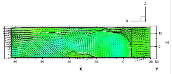
Figure 12: Comparison of the velocity fields obtained in the XZ plane with scanning (in black) and tomo-PIV (in white). The velocity fields represented are tangential and the iso-contours represents the velocity component perpendicular to the plane.
