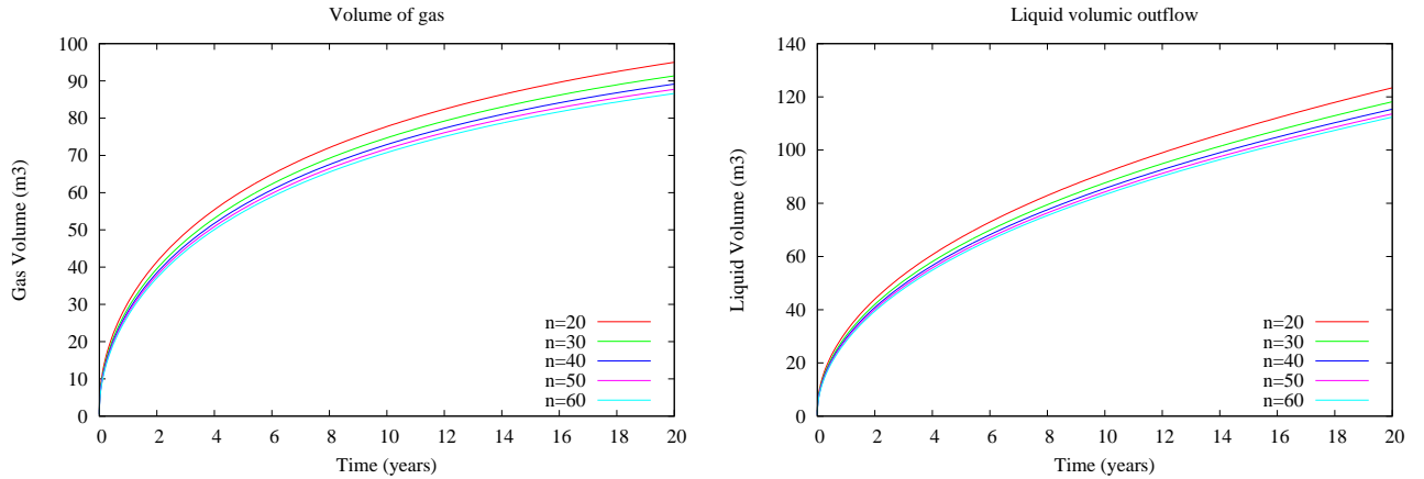
Figure 11: For each mesh n = 20, 30, 40, 50, 60 : volume of gas in the porous media as a function of time, and volumic cumulative outflow of liquid in the gallery function of time.
