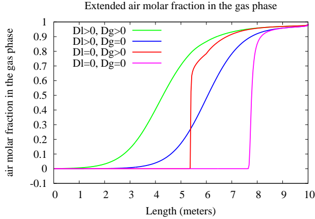
Figure 4: Extended air molar fraction in the gas phase \tilde{c}_a^g in the four cases (i) D^l = D^g = 0 \text{ m}^2 \cdot \text{s}^{-1} ; (ii) D^l = 0 \text{ m}^2 \cdot \text{s}^{-1} , D^g = 10^{-7} \text{ m}^2 \cdot \text{s}^{-1} ; (iii) D^l = 3 \cdot 10^{-9} \text{ m}^2 \cdot \text{s}^{-1} , D^g = 10^{-7} \text{ m}^2 \cdot \text{s}^{-1} ; (iv) D^l = 3 \cdot 10^{-9} \text{ m}^2 \cdot \text{s}^{-1} , D^g = 0 \text{ m}^2 \cdot \text{s}^{-1} at time t = 10 years obtained with the mesh N = 559 and the PPF formulation.
