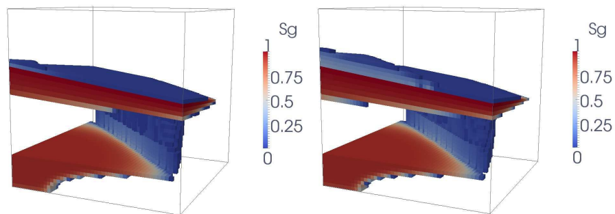
Figure 16: Gas saturation S^g above the threshold 10^{-6} at final time for the PPF (left) and PSF (right) formulations on the mesh 48 \times 48 \times 48 .
