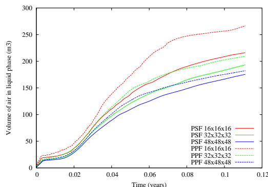
Figure 17: Volume of air dissolved in the liquid phase in the basin function of time for both formulations PSF and PPF and for the family of meshes.
