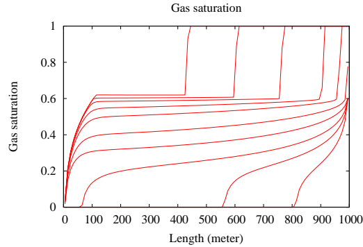
Figure 7: Gas saturation at times t = 1, 3, 6 months, and t = 1, 2, 5, 10, 20, 30, 40 years obtained with the mesh N = 100 and the formulation (P^g, P^l) .
