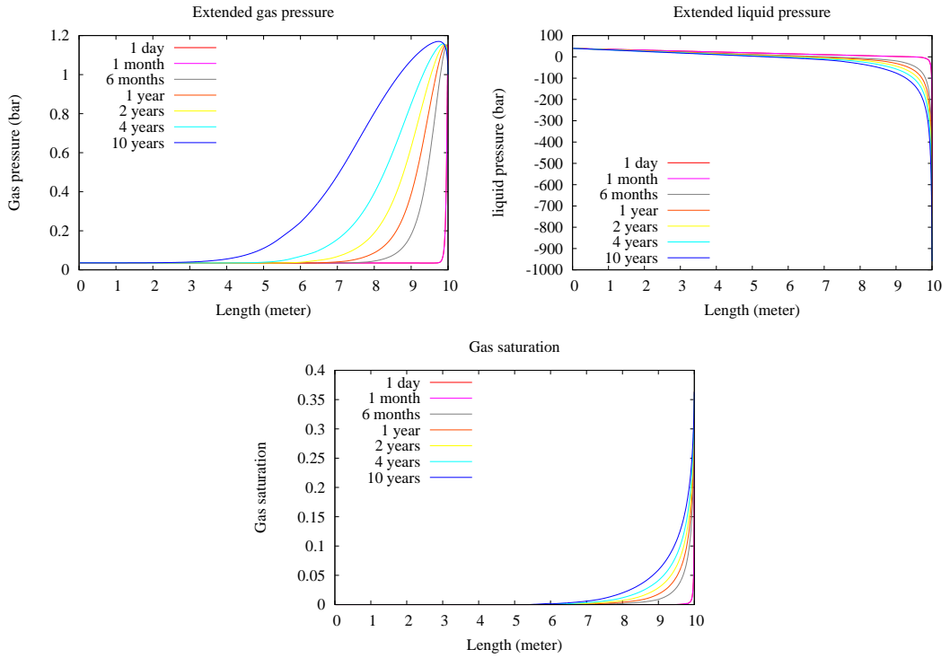
Figure 1: Gas saturation, and extended gas and liquid pressures \tilde{P}^g , \tilde{P}^l at times t = 1 day, 1 month, 6 month, 1 year, 2 years, 4 years, and 10 years obtained with the mesh N = 559 and the formulation PPF .
