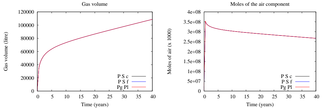
Figure 8: Comparison of the gas volume and the number of moles of the air component at time t = 40 years obtained with the mesh N = 20 and the three formulations PPF, PSF and PSC.
