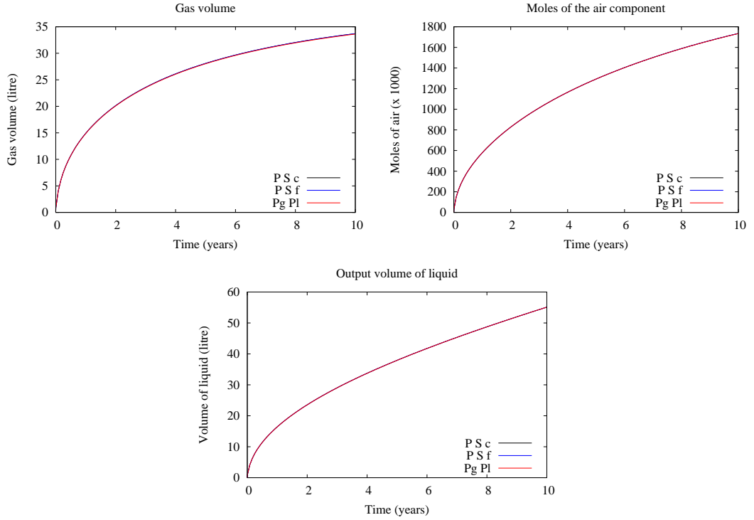
Figure 4: Comparison of the gas volume, the number of moles of the air component, and the output volume of liquid at time t = 10 years obtained with the mesh N = 27 and the three formulations PPF, PSF and PSC.
