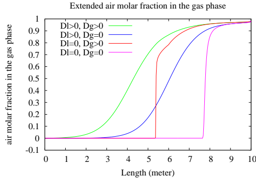
Figure 3: Extended air molar fraction in the gas phase \tilde{c}_a^g in the four cases D^l = D^g = 0 ; D^l = 0, D^g = 10^{-7} ; D^l = 3 \cdot 10^{-9}, D^g = 10^{-7} ; D^l = 3 \cdot 10^{-9}, D^g = 0 at time t = 10 years obtained with the mesh N = 559 and the formulation PPF .
