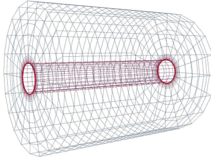
Figure 10: Radial mesh for n = 20 with the EDZ rocktype in red.
