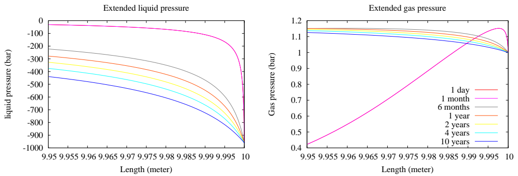
Figure 2: Extended gas and liquid pressures \tilde{P}^g , \tilde{P}^l at the gallery boundary at times t = 1 day, 1 month, 6 month, 1 year, 2 years, 4 years, and 10 years obtained with the mesh N = 559 and the formulation PPF .
