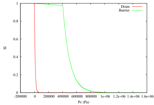
Figure 14: Inverses of the monotone graphs of the capillary pressure in the barrier and in the drain.
