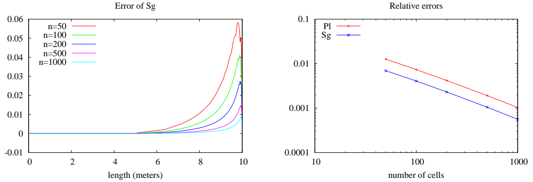
Figure 5: Convergence of the discrete gas saturation S^g and liquid pressure P^l obtained at large times to the stationary analytical solutions for the family of uniform meshes N = 50, 100, 200, 500, 1000 and the PPF formulation. The results obtained with the two other formulations are the same.
