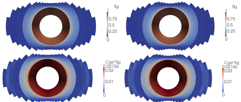
Figure 11: Transversal cut of S^g and of S^g c_e^g at final time obtained on the mesh n = 60 for the PPF formulation (left) and the PSF formulation (right).
