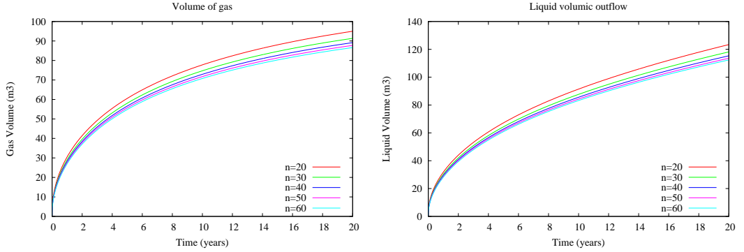
Figure 12: For each mesh n = 20, 30, 40, 50, 60 : volume of gas in the porous media function of time, and volumic cumulative outflow of liquid in the gallery function of time.
