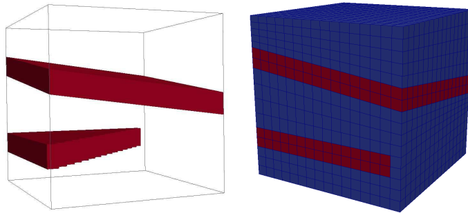
Figure 15: Basin domain with the two barriers in red and the surrounding drain. Mesh 16 \times 16 \times 16 of the basin.
