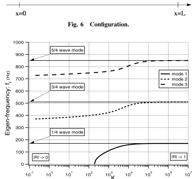
Fig. 7 Eigenfrequencies of the first three modes vs K for the duct of Fig. 6.
