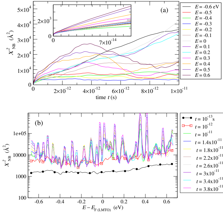
Figure 3. (color online) LMTO non-Boltzmann average square spreading X_{\text{NB}}^2 in \lambda\text{-Al}_{4.6}\text{Mn} . (a) X_{\text{NB}}^2 versus time t for various energy values, (b) X_{\text{NB}}^2 versus energy E for various time values.
