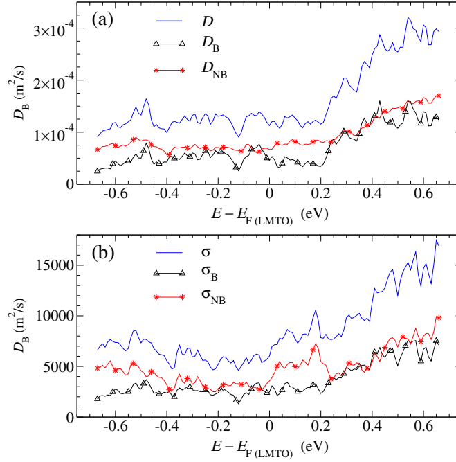
Figure 4. Electronic (a) diffusivity and (b) conductivity in \lambda -Al 14.6 Mn calculated from ab-initio LMTO method for scattering time \tau = 10^{-13} s.
