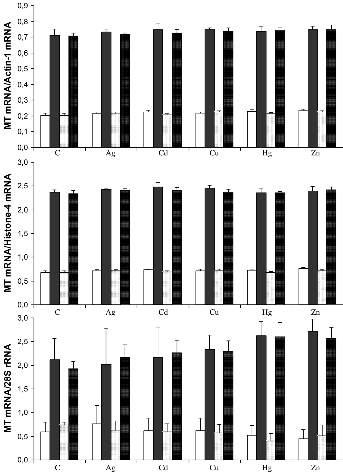
Figure 6. Normalised levels of MT mRNA in the gills (□ : MT-10 and ■ : MT-20) and in the mantle (▤ : MT-10 and ▥ : MT-20) of Bathymodiolus thermophilus at the atmospheric pressure. Mussels were exposed to various metals at different concentrations (see table 3) during 44 hours. C is for Control. The data represent means \pm S.D. with n=10.
