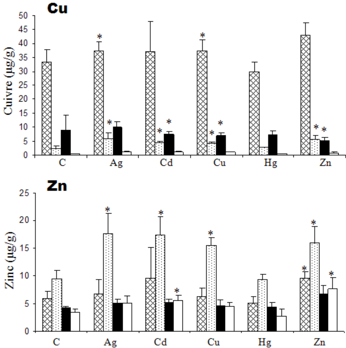
Figure 5. Subcellular distribution of metals (Cu, Zn) in soluble and pellet fractions obtained after the centrifugation of gills (⊠: insoluble fraction, ⊞: soluble fraction) and mantle (■: insoluble fraction and □: soluble fraction) homogenates (mean ± S.D., n=10, \mu\text{g g}^{-1} w.w.). Asterisks indicate significant differences ( P \leq 0.05 ) between control (C) and exposed mussels (Ag, Cd, Cu, Hg, Zn) as determined by Kruskal–Wallis tests.
