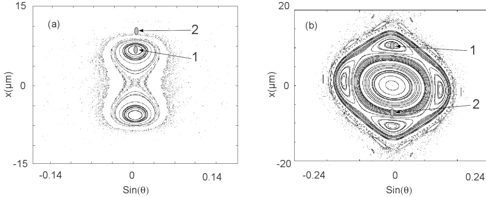
Fig. 2. Poincaré section of the waveguide that exhibits 2 resonances surrounded by a chaotic sea (a). Waveguide parameters are \delta n = 0.024 , \Lambda = 300\mu\text{m} , the waveguide width is w = 12.3\mu\text{m} and the DC = 0.8 . Poincaré section for a different waveguide configuration that exhibits 4 peripheral resonances surrounded by closed curves corresponding to stable trajectories (b). Waveguide parameters are \delta n = 0.05 , \Lambda = 146\mu\text{m} , the waveguide width is w = 15\mu\text{m} and the DC = 0.8 .
