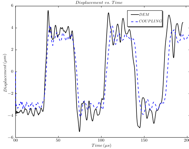
Figure 22: Test4: The free-end displacement U_{x \text{ mean}} obtained by DEM and the coupling method L_O = 10 \text{ mm} , coarse Multiplier space, continuous differentiable weight functions, \varepsilon = 0.05
