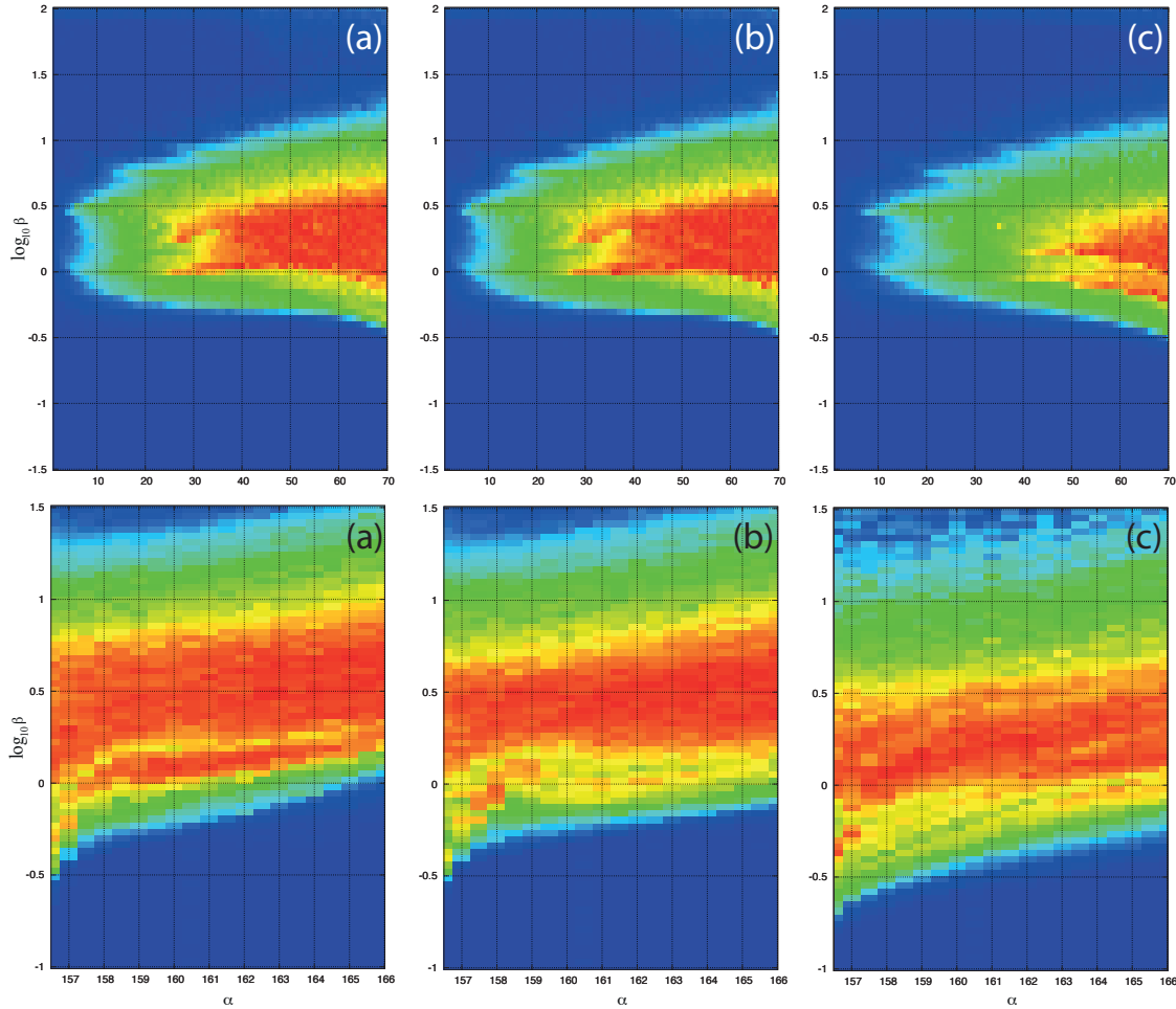
FIG. 6.— Same plots as in Figure 1 ( m/m_c = m_c/m_0 = 10^{-3} ), but for different mass ratios. Top pictures correspond to tadpole-type orbits (\alpha, \log_{10} \beta) \in [0^\circ : 70^\circ] \times [-1.5 : 2] , while bottom pictures correspond to horseshoe type orbits (\alpha, \log_{10} \beta) \in [156^\circ : 166^\circ] \times [-1 : 1.5] . We fix m_c/m_0 = 10^{-6} and vary m/m_c : (a) m/m_c = 10^{-3} ( \delta = 0.999 ); (b) m/m_c = 0.1 ( \delta = 10/11 ); (c) m/m_c = 1 ( \delta = 1/2 ).
