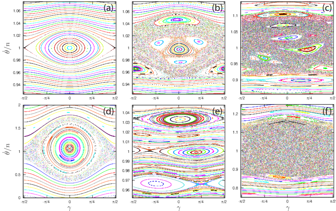
FIG. 4.— Poincaré surface sections in the plane (\gamma, \dot{\theta}/n) deduced from the time- 2\pi/\nu map of the flow (Eq. 4). The angle \gamma is reduced modulo \pi . In the top graphs we fix \beta = 1 and increase the amplitude \alpha : (a) \alpha = 0^\circ . In this case, the dynamics is the same as a simple pendulum for all \beta ; (b) \alpha = 10^\circ . Although the super and sub-synchronous islands are small (Eq. 10), the partial overlap of the resonances already generate a significant chaotic region; (c) \alpha = 50^\circ . For large amplitudes, the islands' overlap give rise to a huge unstable region surrounding the synchronization. In the bottom graphs we fix \alpha = 50^\circ and vary \beta : (d) \beta = 10^{1-3} . The three islands merged generating a chaotic layer in the neighborhood of the synchronization separatrix, as for the modulated pendulum; (e) \beta = 10^{-0.4} . The three main resonant islands are isolated, narrow chaotic regions are present along the associated separatrices; (f) \beta = 10^{0.4} . Deep inside the chaotic zone, in this case no stable motion is possible.
