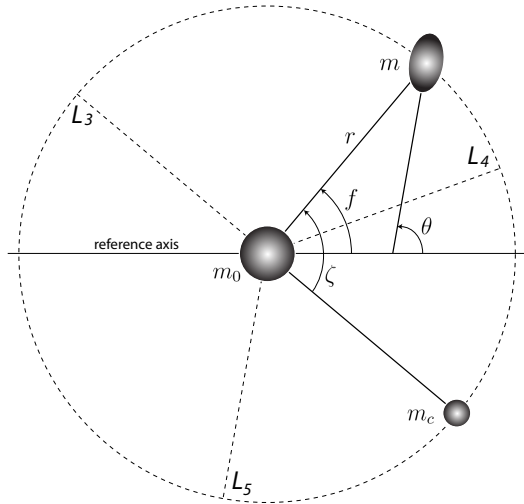
FIG. 1.— Reference angles for the coorbital system. m_0 is the mass of the central body, m the mass of the rotating body, and m_c the mass of the coorbital companion. \theta is the rotation angle of m , r its distance to the central body, and f its true anomaly. \zeta is the angle between the directions of m_c and m .
