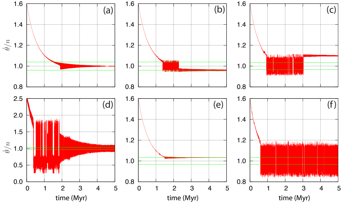
FIG. 5.— Examples of the final evolution of the rotation of a coorbital body. We numerically integrate the equations (1–4) with n = 17.78 \text{ yr}^{-1} (corresponding to m_0 = 1 M_\odot and r_0 = 0.5 \text{ AU} ), together with tidal dissipation using K = 250 \text{ yr}^{-1} (Eq. 7). We show an example for each pair (\alpha, \beta) taken from Fig. 4. The initial rotation rate is \dot{\theta}/n = 2.5 in (d) and \dot{\theta}/n = 1.6 in all the other plots. The green dotted lines give the position of the super- and sub-synchronous resonances n \pm \nu/2 (Eq. 10).
