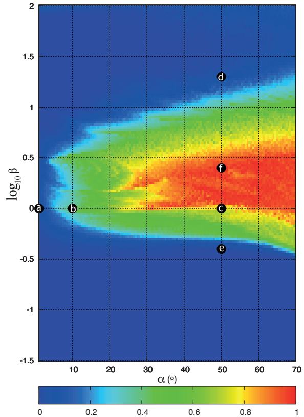
FIG. 3.— Stability analysis of the rotation rate close to the synchronization for (\alpha, \log_{10}\beta) \in [0^\circ : 70^\circ] \times [-1.5 : 2] (Tadpole orbits). The color index indicates the proportion of chaotic orbits inside the studied domain: from dark blue for fully regular to red for entirely chaotic. Above the chaotic region ( \log_{10}\beta > 0 ) only synchronous rotation is possible, while below it ( \log_{10}\beta < 0 ) several spin-orbit resonances are possible. In this plot we fixed \mu \simeq m_c/m_0 = 10^{-3} and m/m_c = 10^{-3} , but these values do not significantly affect the results as long as m/m_c < 0.1 (Fig. 6). The black circles correspond to the locations of the six examples presented in Figures 4 and 5.
