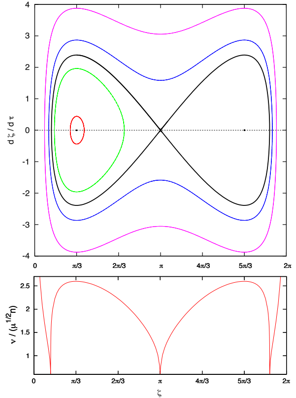
FIG. 2.— Longitudinal variations of coorbital bodies (Eq. 14) in the plane (\zeta, d\zeta/d\tau) (top), and orbital libration frequency taken over the dashed line ( \nu versus \zeta with d\zeta/d\tau = 0 ) (bottom). The black curve is the separatrix between the tadpole and the horseshoe orbits ( \zeta_{\min} \approx 24^\circ ). The two tadpole orbits surrounding L_4 correspond to \alpha = 10^\circ and \alpha = 50^\circ , while the two horseshoe orbits are associated to \alpha = 160^\circ and \alpha = 166^\circ .
