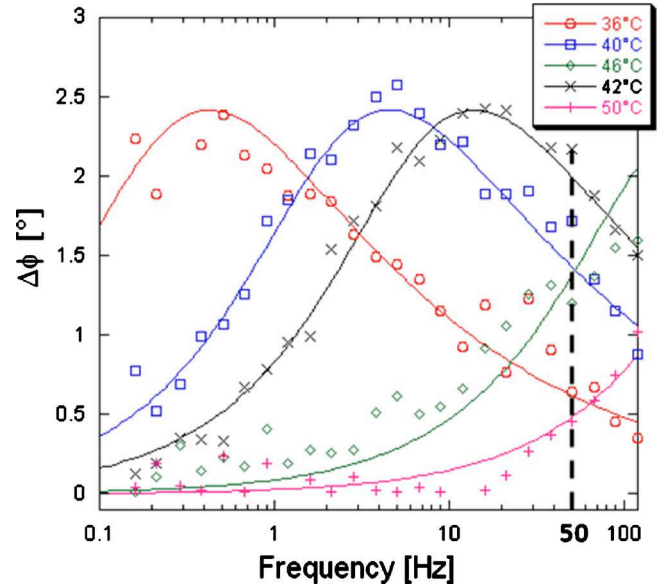
FIG. 2. (Color online) Phase shift measured as a function of the frequency over an island of PVAc. Statistical error is 0.25 for f>1 Hz and 0.35 for f\leq 1 Hz. Lines are fits derived from a KWW model with amplitude and shape parameters fixed for all curves. The dashed line indicates the imaging frequency of Fig. 3.
