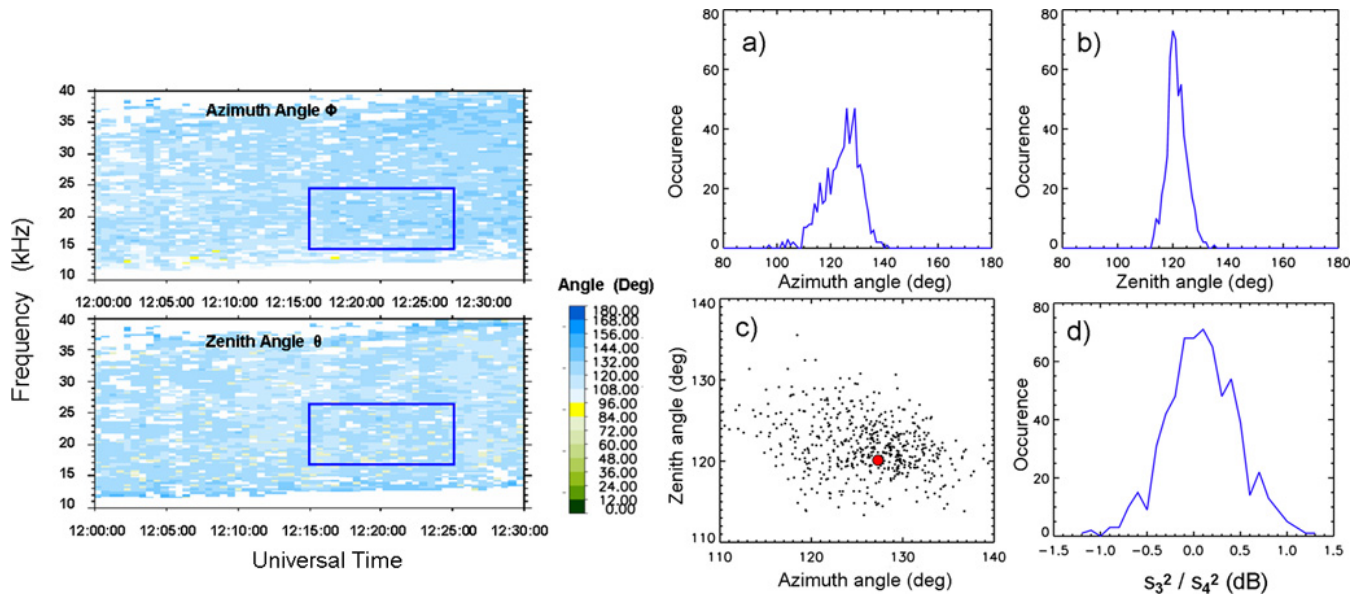
Fig. 7. DSM tool applied to a frequency–time domain during 18 May 2008 event. Elementary runs treat the signal at a fixed frequency bin (320 Hz width) measured on C3 and C4 during an interval of 60 s. Left: frequency–time spectrograms of derived ray path vector orientation angles (azimuth and zenith) in GSE coordinate system. Right: distribution of quantities derived from the runs inside the pointed frequency–time domain (blue rectangle); (a) azimuth angle occurrence, (b) zenith angle occurrence, (c) zenith versus azimuth, and (d) ratio of electric field powers measured on C3 and C4 along the common antenna orientation.
