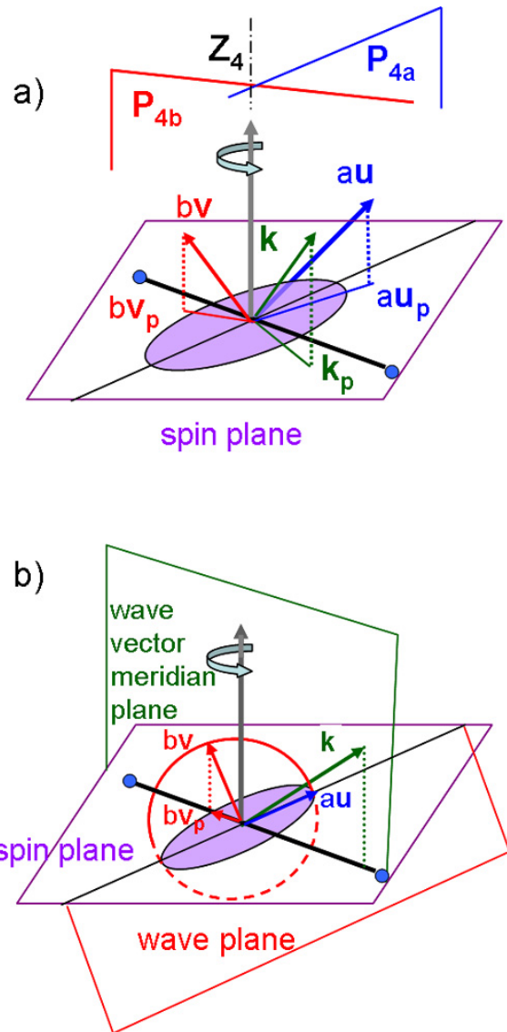
Fig. 3. Case of elliptic polarization. (a) Linear components au and bv of an electric field elliptically polarized. Vectors u and v of the wave plane and its normal k are shown in [S_{C4}] coordinate system. Meridian planes P_{4a} and P_{4b} contain Z_4 axis and, respectively, u and v vectors. Projections u_p, v_p and k_p of u, v and k onto C4 spin plane are shown, as well as the electric field ellipse projected onto the same plane (purple area). (b) Specific case of circular polarization where principal axis positions have been chosen such that u vector was in the spin plane. Projections u_p ( u_p = u ) and v_p are at a right angle to each other. The meridian plane (drawn in green) formed by the spin axis and v_p contains the wave vector k .
