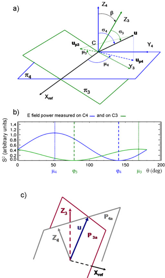
Fig. 2. Case of linear polarization. (a) Sketch of unit vector u of an electric field vector of magnitude a in the tilted pair system. The orientation of u is defined by the two angles, \sigma_4 and \mu_4 in spherical coordinates of the [S_{C4}] system, alternatively \sigma_3 and \mu_3 in the [S_{C3}] coordinate system. Vectors u_{p4} and u_{p3} are projections of vector u onto spin planes. (b) Electric field power variations plotted versus antenna attitudes angles in a chosen case (see text). They reach a maximum when the antenna is aligned with u_{p4} and u_{p3} (attitude angles \mu_4 and \mu_3 ), and is null when the antenna is at right angles to the projections (angles \phi_4 and \phi_3 ). (c) The two meridian planes P_{4a} and P_{3a} , attached respectively to [S_{C4}] and [S_{C3}] coordinate systems, intersecting along vector u .
