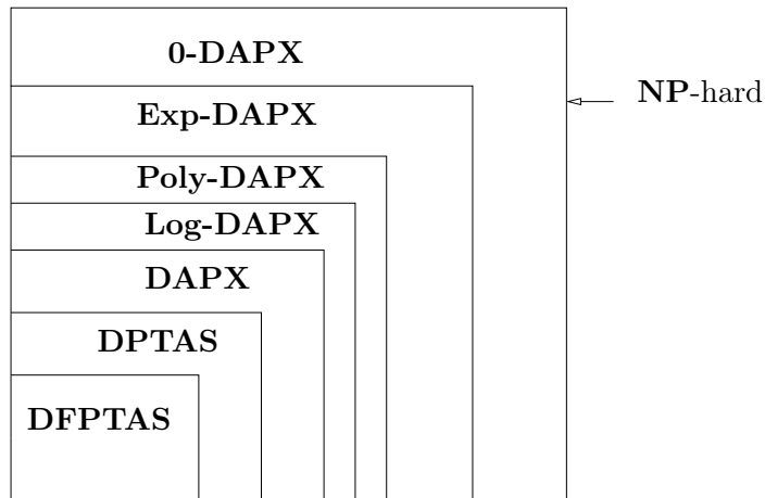
Figure 2: Differential classes (under the assumption \mathbf{P} \neq \mathbf{NP} ).
