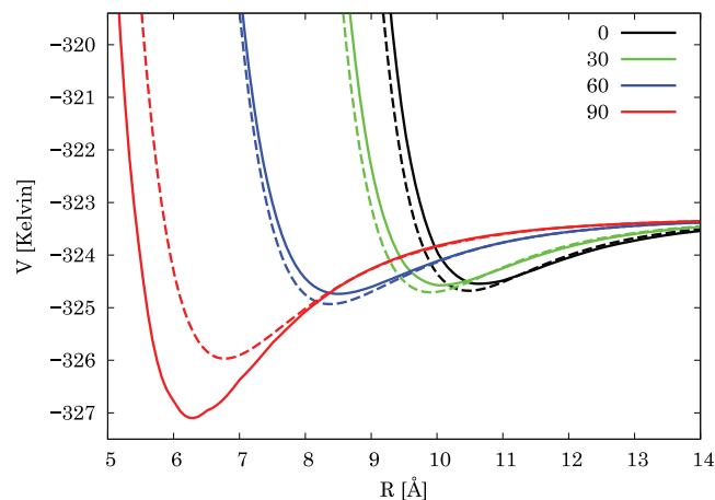
FIG. 1. Cuts of the potential energy surface at r = 6.117 \text{ \AA} for \gamma = 0^\circ (black), 30^\circ (green), 60^\circ (blue), and \gamma = 90^\circ (red) in Kelvin as a function of R . The full potential surface is presented in full lines while the restriction to the two-body expansion is shown in dashed lines. The zero of energy corresponds to the separated atoms limit.
