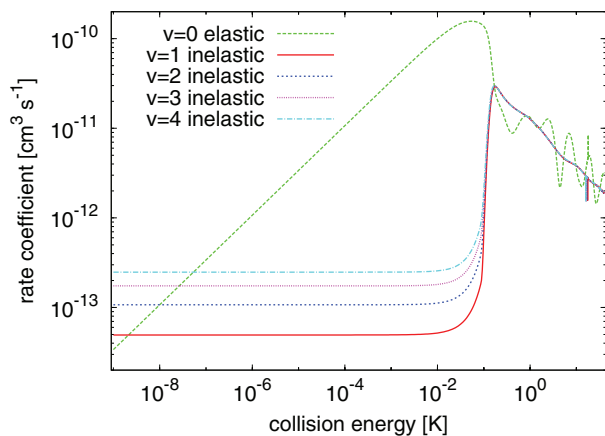
FIG. 6. Elastic and inelastic J = 0 rate coefficients for 4 He + Rb 2 collisions with the initial rovibrational state v_i = 0, \dots, 4, j = 0 of Rb 2 as a function of the collisional energy in Kelvin.
