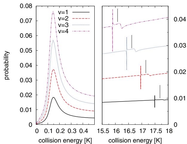
FIG. 4. Vibrational relaxation probability for {}^4\text{He} as a function of collision energy in Kelvin for initial rovibrational states (v_i, j_i = 0) with v_i = 1, 2, 3 , and 4. This figure presents two blow-ups of the data presented in Fig. 3 in the energy ranges of the two resonance features. The openings of the (v_i + 1, j = 0) channels are materialized by the vertical black lines in the right panel.
