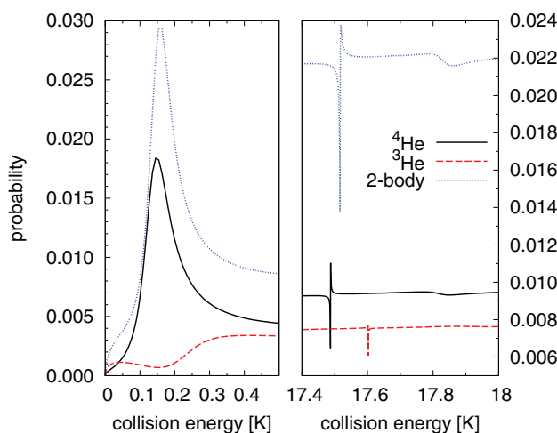
FIG. 5. Vibrational relaxation probability for v_i = 1 as a function of collision energy in K. The black full line corresponds to {}^4\text{He} colliding with \text{Rb}_2 using the full potential. The red dashed line presents the effect of the isotopic substitution of {}^4\text{He} by {}^3\text{He} on the full potential. The blue pointed line is obtained when {}^4\text{He} collides with \text{Rb}_2 on the two-body potential surface.
