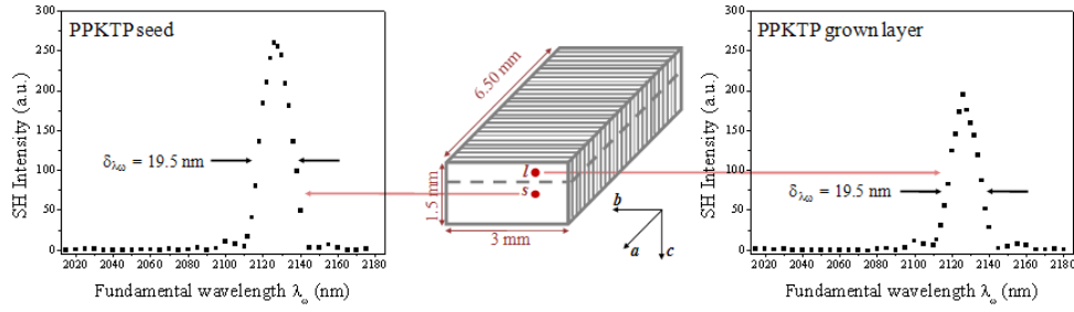
Fig. 5. Comparison between the quasi-phase matched second harmonic generation (QPM SHG) properties of the seed and one side of the grown layer at room temperature. QPM SHG measurements performed at two different depths, 275 \mu\text{m} in the seed ( s ) and 225 \mu\text{m} in the epitaxial layer ( l ) measured from the interface (dashed line) in a sample with a grating periodicity \Lambda = 38.86 \mu\text{m} .
