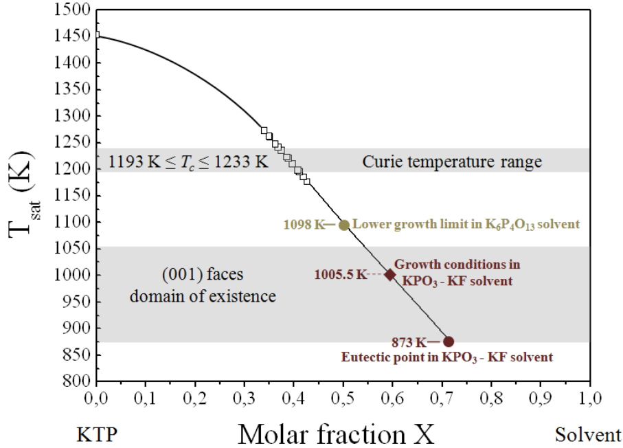
Fig. 3. The pseudo-binary phase diagram of KTiOPO_4 (KTP) using K_6P_4O_{13} and 4KPO_3 : 2KF solvents. T_{sat} is the saturation temperature of KTP below which the crystallization can occur; X is the molar fraction defined by [K_6P_4O_{13}]/\{[KTP]+[K_6P_4O_{13}]\} or [4KPO_3 : 2KF]/\{[KTP]+[4KPO_3 : 2KF]\} according to the considered solvent.
