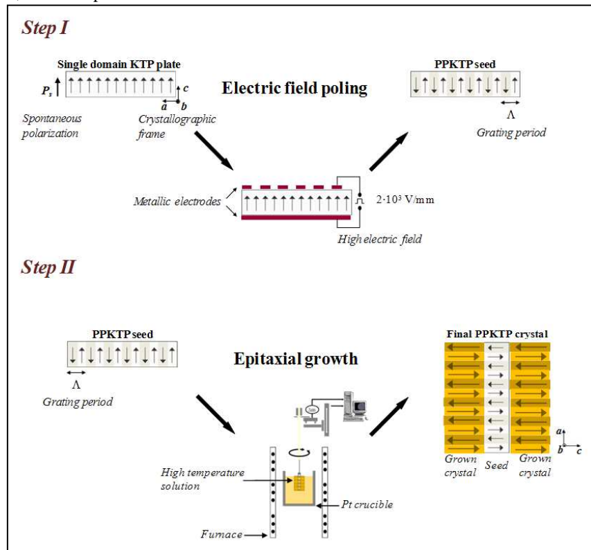
Fig. 1. Scheme of the process showing the different steps to obtain large size PPKTP crystals. Step I corresponds to the fabrication of a PPKTP sample from a single domain KTP plate by electric field poling. Step II corresponds to the growth of a large size PPKTP crystal from the PPKTP seed by the flux method.
