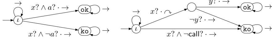
Fig. 6. Automata for P_a(x) and x \rightsquigarrow y
