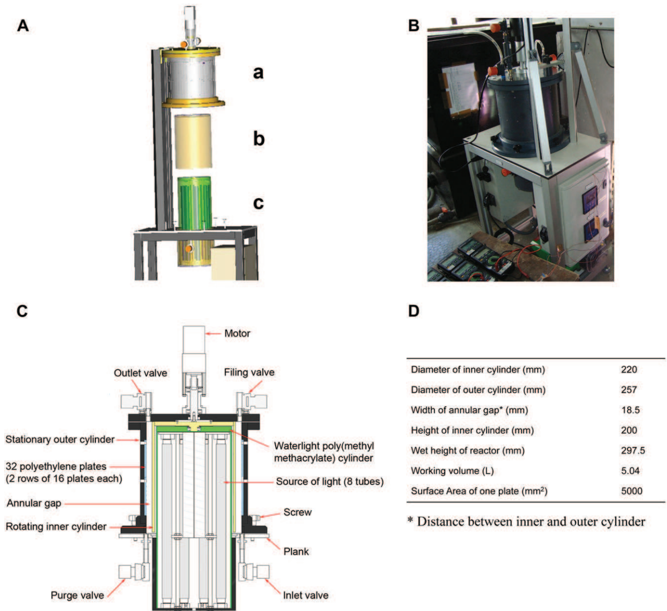
Fig. 1 – Setup of the photosynthetic rotating annular reactor (RAB) with Taylor–Couette type flow. (A) 3D representation of different parts composing the RAB, a : the stationary outer cylinder, b : the rotating inner cylinder and c : the light source protected by an internal water-tight cylinder, (B) photograph of RAB, (C) schematic diagram of RAB and (D) geometric characteristics of RAB.
