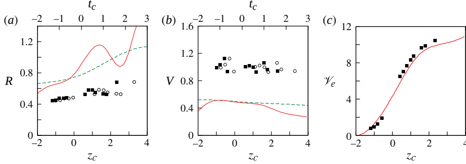
FIGURE 15. (Colour online) Evolution of (a) the normalized ring radius R , (b) rise speed V , and (c) entrained volume V_e for the toroidal bubble displayed in figure 13 versus the dimensionless vertical position z_c of the bubble's centre of inertia above the undisturbed interface (black squares and solid line). Subfigures (a) and (b) also display the corresponding evolutions versus the dimensionless time t_c , with t_c = 0 when z_c = 0 (open circles and dotted line). The 'experimental' ring and core radii are obtained by evaluating the dimensionless area S^* and perimeter P^* of the projected surface \mathcal{S} of the bubble on images such as that of figure 14, and equating these quantities with their counterparts for a torus with a circular core, which yields the conditions S^* = 4Ra + \pi a^2 and P^* = 4R + 2\pi a ; the rise velocity is defined as the time variation of the vertical position of the centre of inertia of \mathcal{S} and the entrained volume is obtained by fitting the fluid–fluid interface contour with a curve preserving the left–right symmetry, evaluating the enclosed volume by invoking axisymmetry and removing the known bubble volume; this procedure does not work when the bubble crosses the undisturbed position of the interface, which is why no data appear in (c) during that stage. The computational ring radius is defined as R(t) = \int r^2 C(r, z, t) dr dz / \int r C(r, z, t) dr dz , where C is the local volume fraction of air and integration is performed over the whole computational domain; the rise velocity is defined as V(t) = \int r U_z(r, z, t) C(r, z, t) dr dz / \int r C(r, z, t) dr dz , where U_z is the local vertical fluid velocity.
