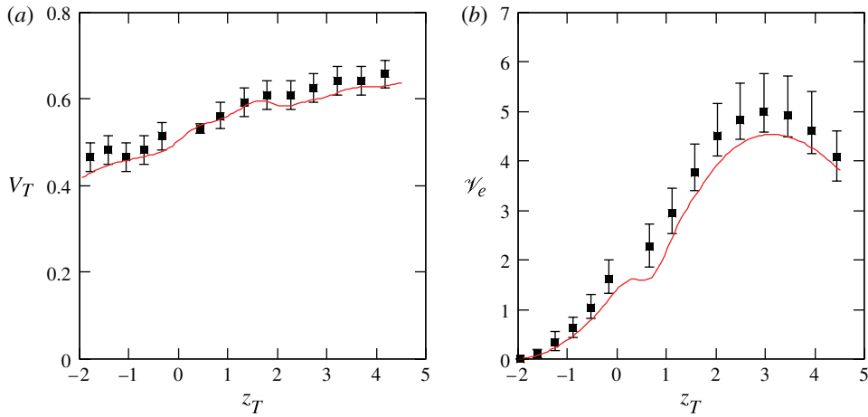
FIGURE 9. (Colour online) Evolution of (a) the normalized rise speed V_T and (b) the displaced volume \mathcal{V}_e for the bubble considered in figure 8. See figure 5 for legend.
