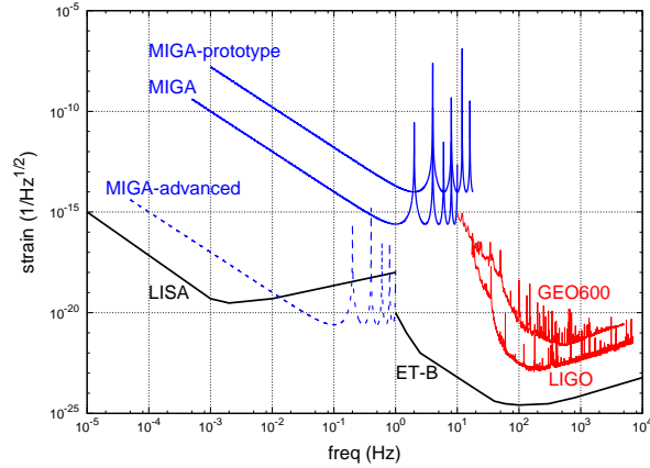
Fig. 31. – Comparison of strain sensitivity curves of different generations of atom-laser interferometers and the optical counterpart. The blue curves, relative to MIGA–prototype and MIGA, consider current technology ( T = 0.25 s and 0.5 s, respectively; 4\hbar k beam-splitters; L = 10 m and 400 m, respectively; signal-to-noise ratio = 10^{-3} ). The dashed MIGA–advanced curve is the projected sensitivity assuming a trapped sample ( T = 5 s), LMT beam-splitters ( 400\hbar k ), and improved sensitivity from a large number of atoms and squeezed states. In red, the sensitivity curves of LIGO and GEO600—two operational Earth-based optical GW detectors. In black is the projected sensitivity of future optical GW detectors: the space-based LISA, and the underground Einstein Telescope.
