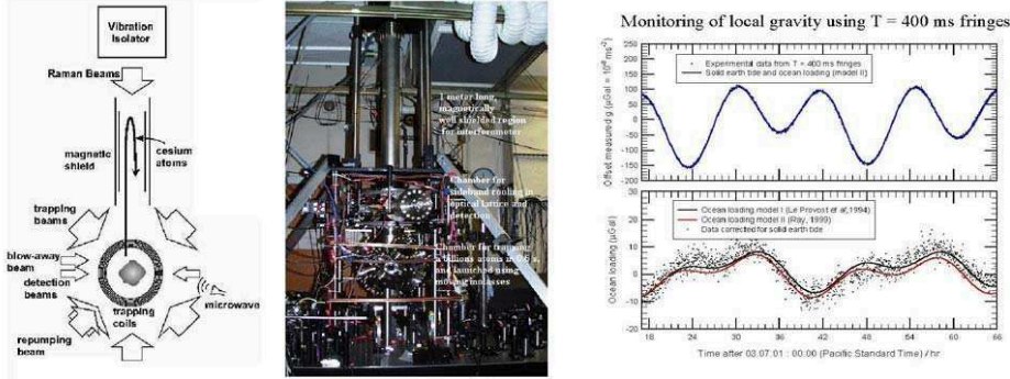
Fig. 9. – Principle of the atom-fountain-based gravimeter achieved by the Chu group at Stanford during the 1990’s [14, 37, 19] . On the right is a two-day recording of the variation of gravity. The high accuracy enables ocean loading effects to be observed. Photo courtesy of S. Chu and M. Kasevich.
