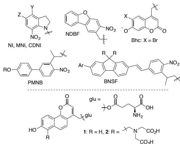
Chart 1. TPA chromophores.
