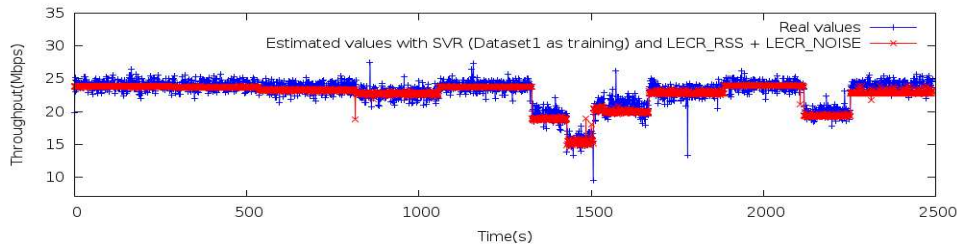
Fig. 2: Throughput estimation results obtained with the LECR\_RSS+LECR\_NOISE metric compared to the real throughput.
