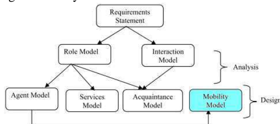
Figure 2: Structure of m-GAIA's models (Sutandiyo et al., 2004).
