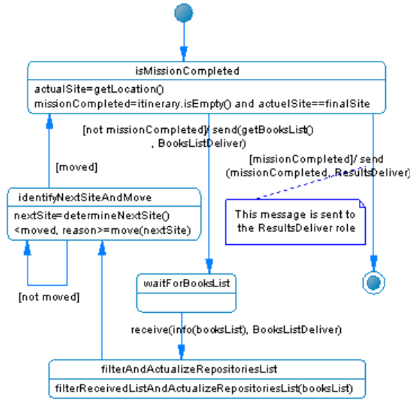
Figure 16: searchBook task.
