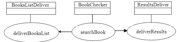
Figure 15: Roles diagram.
