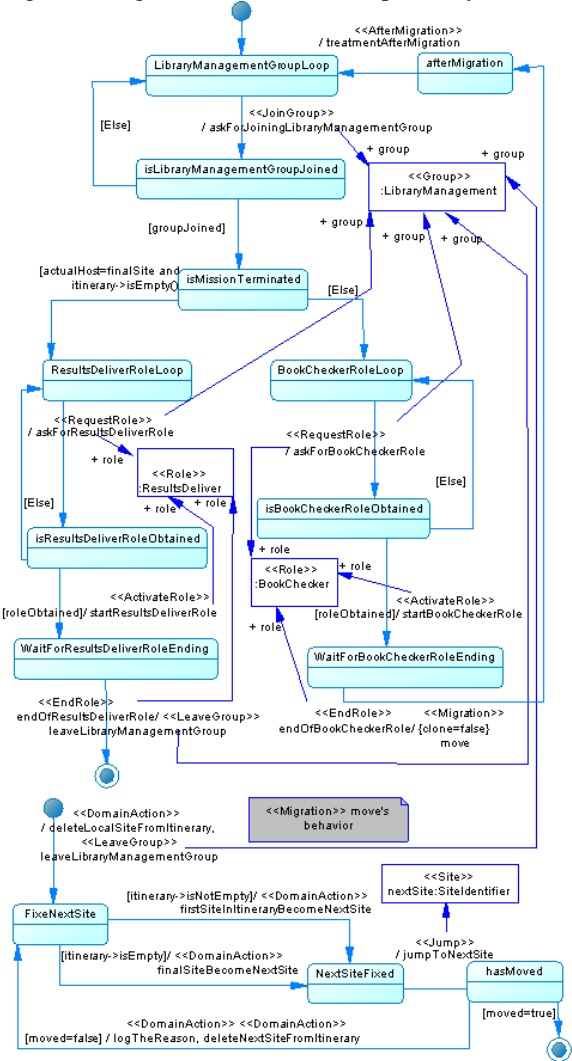
Figure 11: MobileBookSeeker behavior.
