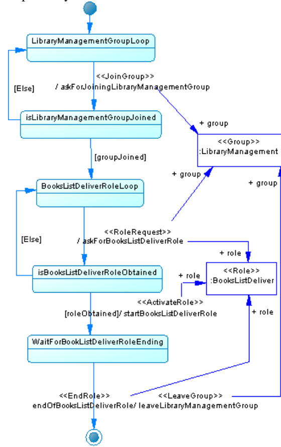
Figure 9: Librarian behaviour.
