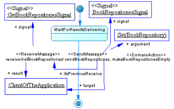
Figure 13: ResultsDeliver behaviour.
