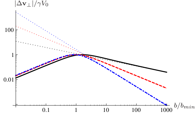
Figure 1. Numerical computation of |\Delta\mathbf{v}_\perp| after a collision, for \gamma = 1/2 (plain curve), \gamma = 1 (dashed curve) and \gamma = 3/2 (dashed-dotted curve). The weak collision approximation for each case is represented with dotted lines, which coincides perfectly with the exact calculations for b \gg b_{min} .
