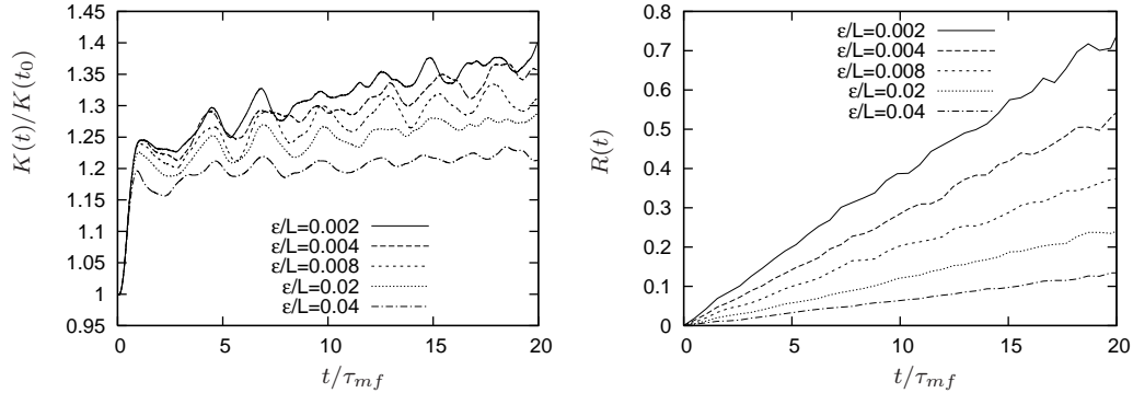
Figure 3. Left: evolution of the total kinetic energy K for simulations with N = 8000 particles and different softening length \epsilon in the potential v(r) with \gamma = 5/4 . Right: evolution of the estimator R(t) for the simulations.
