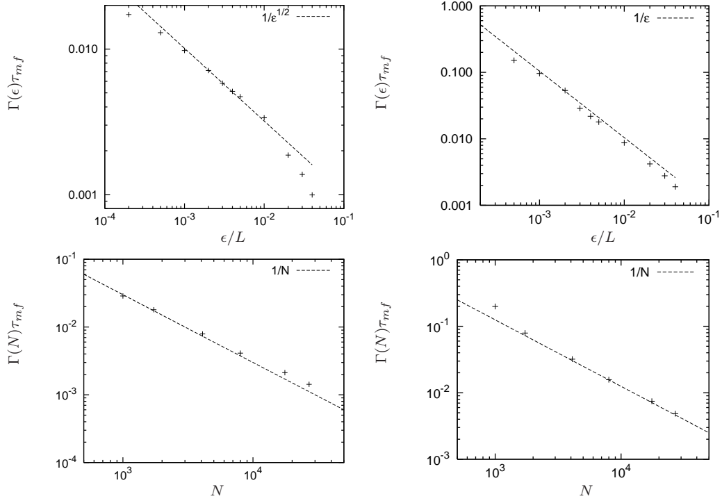
Figure 4. Top left: Relaxation rate estimated using the estimator (32) for N = 8000 , \gamma = 5/4 and different values of the softening \epsilon . Top right: the same plot but for \gamma = 3/2 . Bottom left: relaxation rate for \epsilon/L = 0.01 , \gamma = 5/4 and different number of particles N . Bottom right: the same plot but for \gamma = 3/2 .
