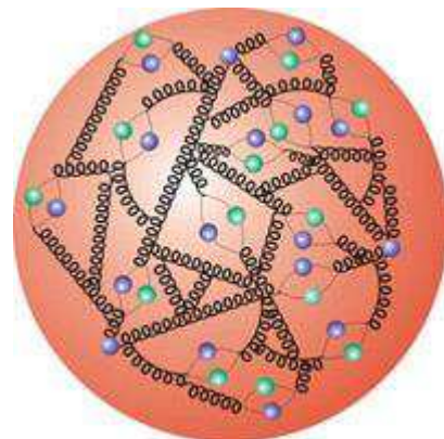
Fig. 1 Inner structure of a proton revealed at HERA. Black spirals represent gluons while purple-green particles denote virtual quark-antiquark pairs (up to 100 of these quark/anti-quark pairs are "visible" at any instant!). Note that there are three more quarks (two up, one down) than anti-quarks. These are the three valence quarks we would normally refer to when speaking of the proton. (Source: DESY in Hamburg)
