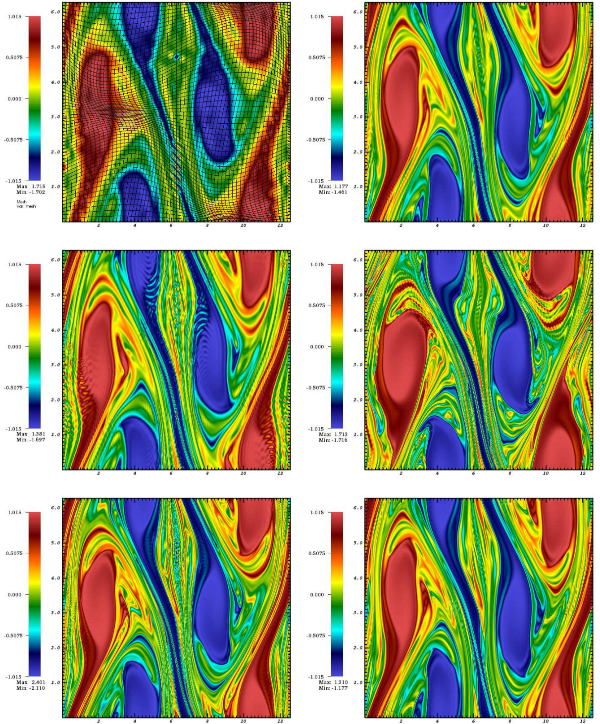
Figure 3: Distribution function f(t = 16, x, y) for different grid sizes, \Delta t and \alpha parameter of the Colella mesh. From left to right, top to bottom: 64 \times 64 , \Delta t = 0.1 , \alpha = 0.7 , 256 \times 256 , \Delta t = 0.1 , \alpha = 0.7 , 256 \times 256 , \Delta t = 0.01 , \alpha = 0.9 , 512 \times 512 , \Delta t = 0.1 , \alpha = 0.9 , 512 \times 512 , \Delta t = 0.01 , \alpha = 0.9 , 256 \times 256 , \Delta t = 0.1 , \alpha = 10^{-6} .
