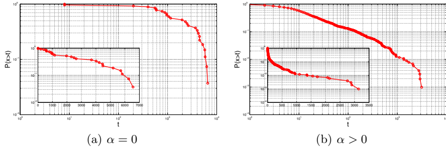
Fig. 2. Theoretical Inter-Contact Time Distribution of STEPS
