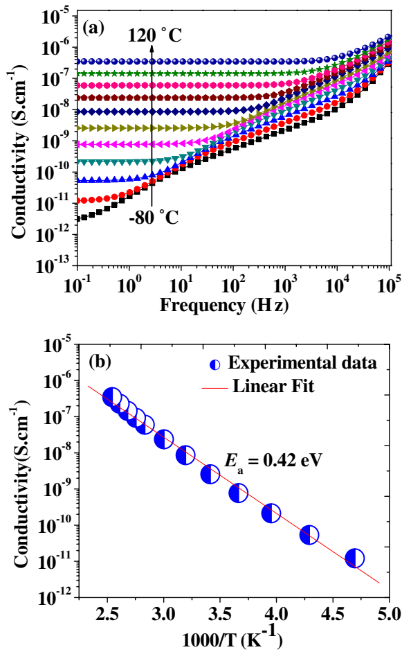
Figure 10. (a) Frequency dependence of the ac conductivity at various temperatures with \Delta T = 20^\circ\text{C} and (b) dc conductivity ( \sigma_{dc} ) as a function of 1000/T .
