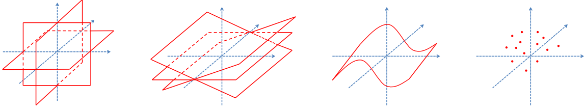
Figure 1: Illustration of several CS models. From left to right: k -sparse vectors, union of subspaces, smooth manifold and point cloud.
