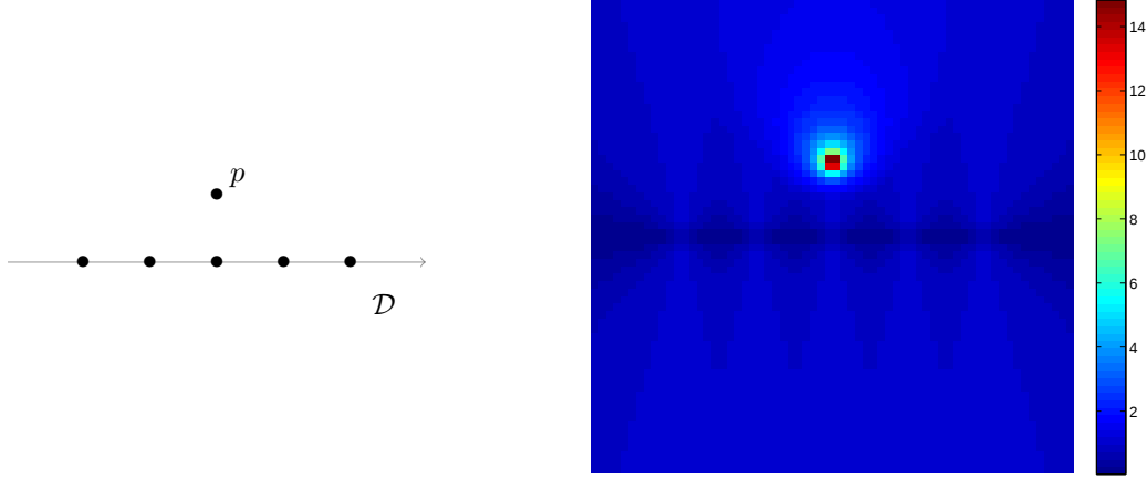
Figure 5: Drawback of uniform instance optimality in a simple case: the model \Sigma (Left) is the set of black points including those on D and the point p and the operator \mathbf{M} is the 1-dimensional orthogonal projection on the horizontal axis. If we choose \Delta as the pseudo-inverse of \mathbf{M} , the depicted IO ratio (Right) is low on most of the space, but the uniform constant is infinite.
