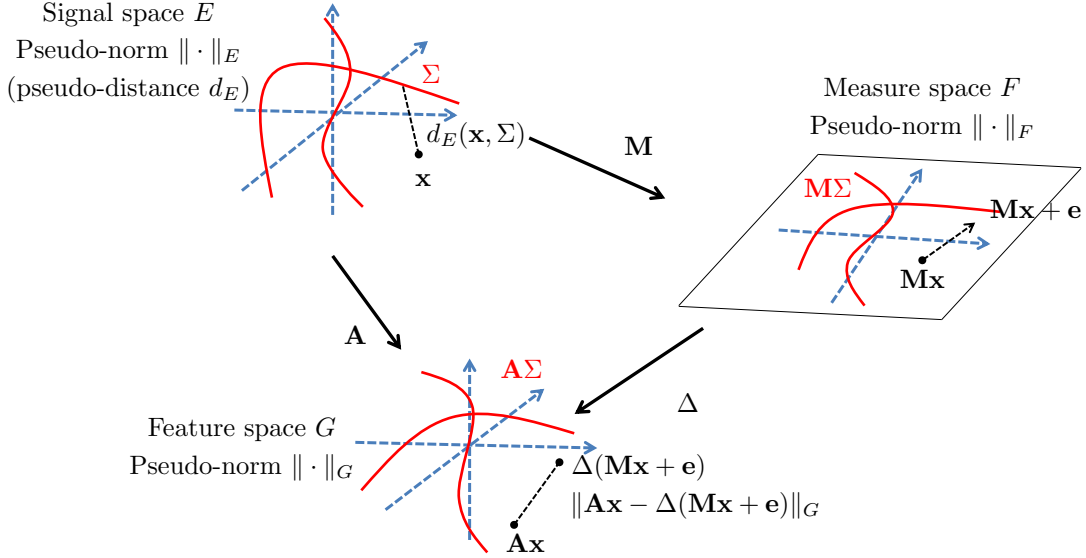
Figure 2: Illustration of the proposed generalized setting. The signals belong to the space E , supplied with a pseudo-norm \|\cdot\|_E used to measure the distance from a vector to the model \Sigma containing the signals of interest. E is mapped in the measure space F by the operator M and the measure is perturbed by an additive noise e . The space F is supplied with a pseudo-norm \|\cdot\|_F . The feature space G , supplied with a norm \|\cdot\|_G , is composed of vectors obtained by applying a linear operator A to the signals in E . These feature vectors are the vectors one wants to reconstruct from the measures in M by applying a decoder \Delta . The reconstruction error for the vector x and noise e is therefore \|Ax - \Delta(Mx + e)\|_G . Note that in the case where E = G and A = I , the decoder is aimed at reconstructing exactly the signals.
