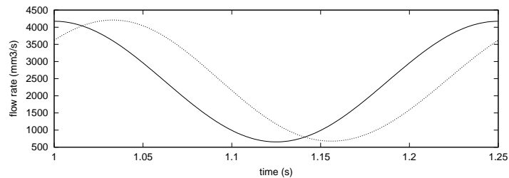
FIGURE 3. Time evolutions of the flow rate at sections — : x = x_{\text{inlet}} and ..... : x = x_{\text{outlet}} for the case R2. Note that the origin of time is 1 s since the fifth cycle is analysed (see text).
