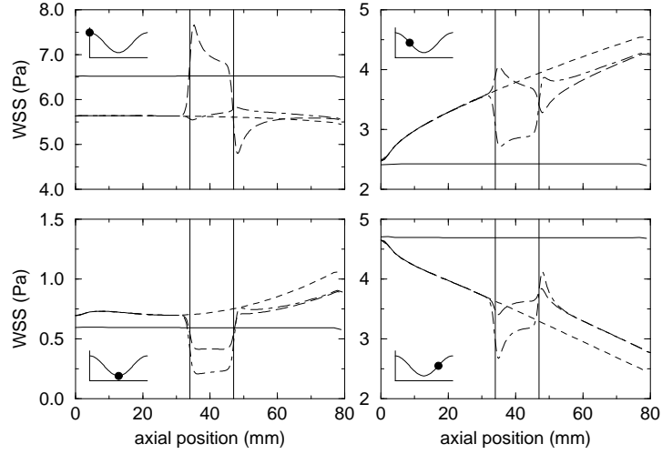
FIGURE 4. Wall shear stress for runs R1 (solid), R2 (dashed), R3 (long dashed) and R4 (dot-dashed) at times: t = nT (systole - top left), t = (n + 1/4)T (top right), t = (n + 1/2)T (diastole - bottom left) and t = (n + 3/4)T (bottom right), where T = 2\pi/\omega is the period. The two vertical lines denote the stent location.
