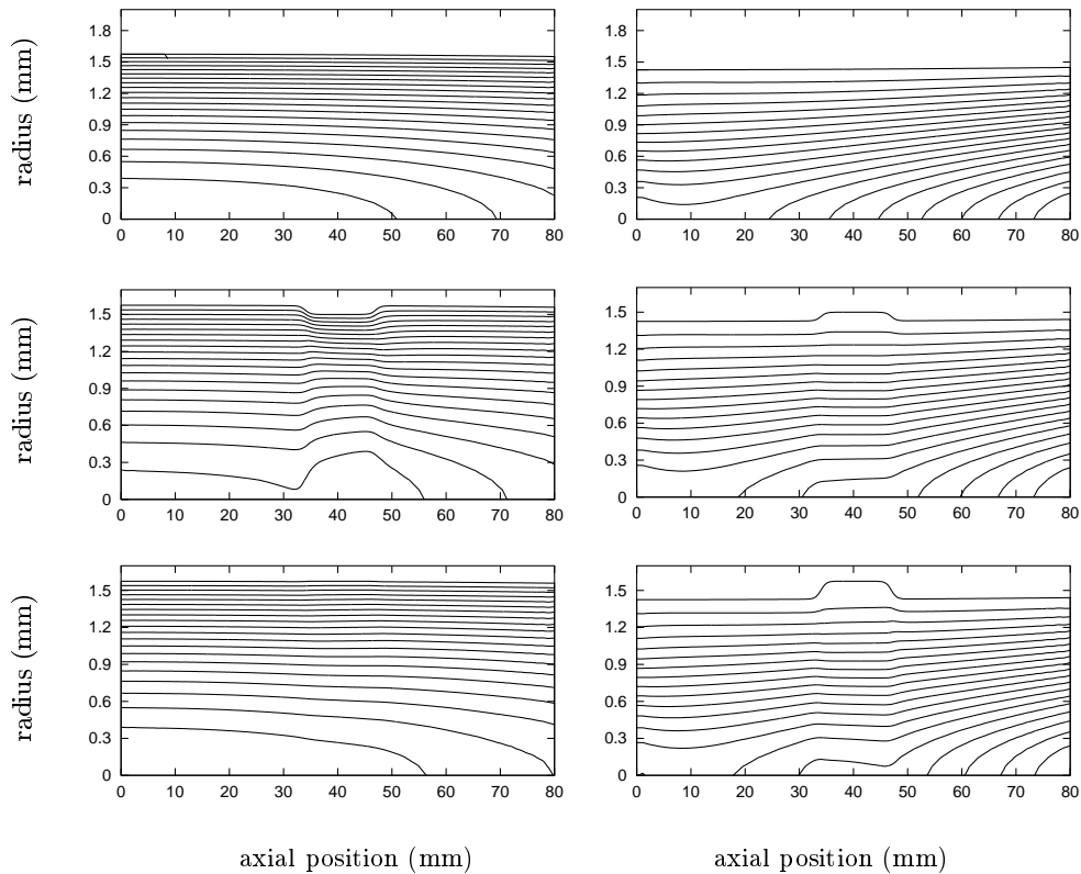
FIGURE 5. Shape of the computational domain at times t = nT (systole - left column) and t = (n+1/2)T (diastole - right column) for the runs R2 (top row), R3 (medium row) and R4 (bottom row). The isolines of the streamwise velocity are plotted. The streamwise and radial coordinates are expressed in millimetres. The aspect ratio R_0/L has been multiplied by 35 for convenience.
