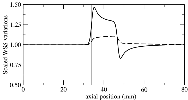
FIGURE 6. Scaled amplitude of the wall shear stress fluctuations for runs R3 (solid) and R4 (long-dashed) The two vertical lines denote the stent location.
