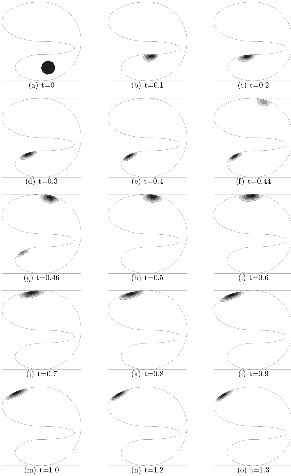
Figure 6: Isolines of rescaled u^\epsilon for different values of t in a non-convex domain
