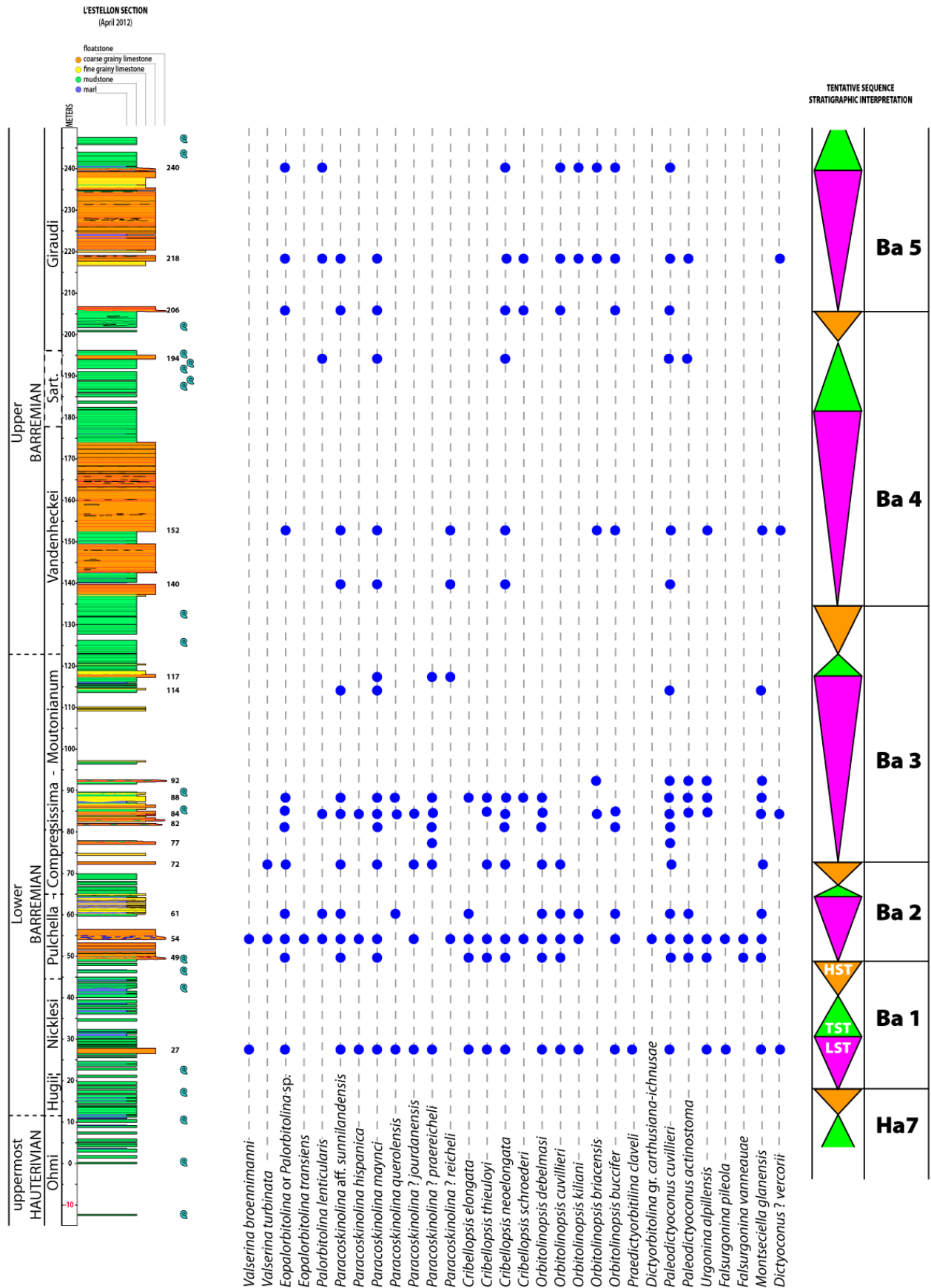
Figure 8: Orbitolinid records together with the latest biostratigraphic interpretation of L'Estellon section as documented by ammonites and planktonic foraminifera (and tentative sequence stratigraphic framework).
