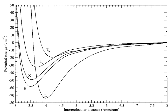
FIG. 3. Potential energy of N 2 -H 2 as a function of the intermolecular distance R for some selected conformations of the dimer: (\theta_A^{N_2}, \theta_B^{H_2}, \varphi) = (90^\circ, 90^\circ, 0^\circ) for H, (0^\circ, 0^\circ, 0^\circ) for L, (90^\circ, 90^\circ, 90^\circ) for X, (90^\circ, 0^\circ, 0^\circ) for T a , and (0^\circ, 90^\circ, 0^\circ) for T b .
