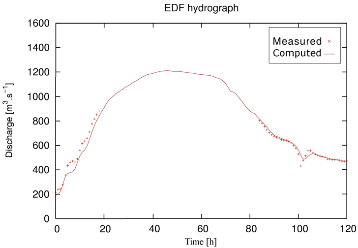
Fig. 7. Measured discharge hydrographs ( m^3s^{-1} ) at the middle gauge station EDF, and computed one using the calibrated model (Manning is calibrated in three land classes, Case b; at downstream, elevation is imposed).
