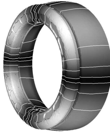
b: Second orthoradial mode - f = 686 Hz
