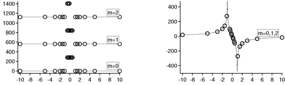
Figure 3. Influence of purely resistive impedance Z = a on the 1D modes eigenfrequencies. Left: real part of the frequency. Right: Imaginary part. \circ numerical results, — analytical solution. Abscissa represent a .
