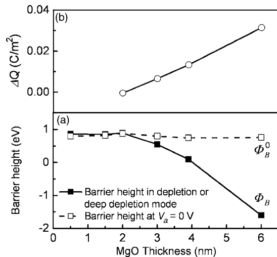
FIG. 3. (a) Evolution of \Phi_B and \Phi_B^0 as a function of the MgO thickness. \Phi_B ( \Phi_B^0 ) corresponds to the barrier height under depletion or deep depletion mode (for the nonpolarized structure). (b) Evolution of the additional positive charge per unit area \Delta Q accumulated in the interface traps [ \Delta Q = C_{OX,A}(\Phi_B^0 - \Phi_B)/e , where C_{OX,A} is the oxide capacitance per unit area and e is the elementary charge].
