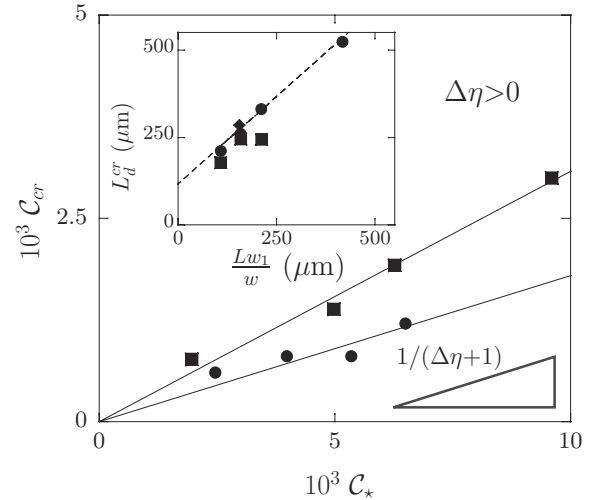
FIG. 4. Evolution of C_{cr} with C , for \Delta\eta > 0 . For both fluid systems, the experimental data collapse onto a single line whose slope is 1/(\Delta\eta + 1) . Inset: Evolution of the critical slug size L_d^{cr} with \frac{Lw_1}{w} . The fluid systems are (■) water in hexadecane, (◆) a viscous water-glucose (28 wt.% glucose) mixture in hexadecane, and (●) a viscous water-glucose mixture (44 wt.% glucose) in hexadecane. The ratio of the widths of the gaps is W = 0.48 . Each data point corresponds to a value of Z = 0.8\text{--}3.8 \times 10^{-3} . The dashed line stands for the linear fit L_d^{cr} = \frac{Lw_1}{w} + 0.9w .
